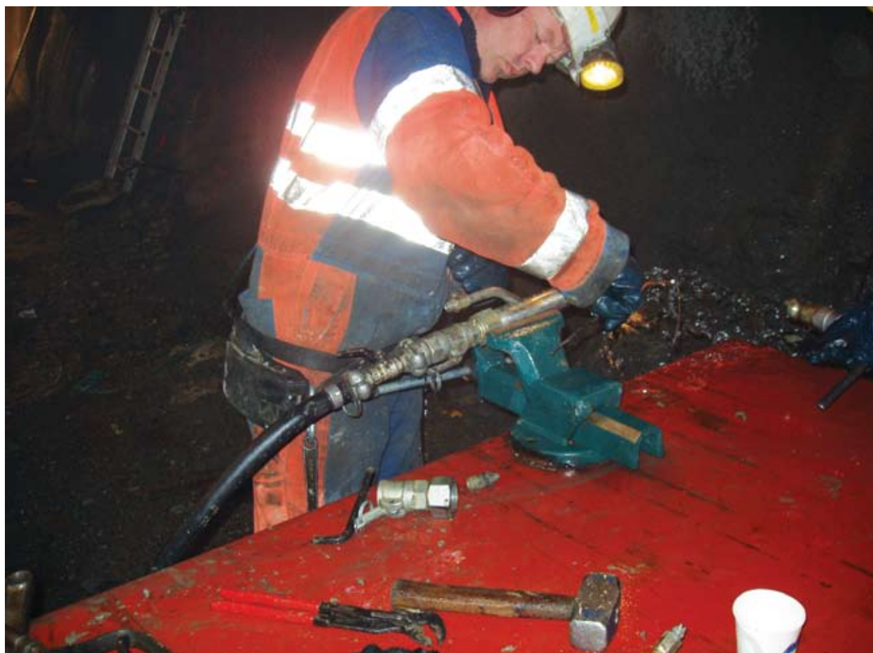
Figure 28. Example of a work bench on a grouting rig. (Photo: John Ivar Fagermo, AF Group)
