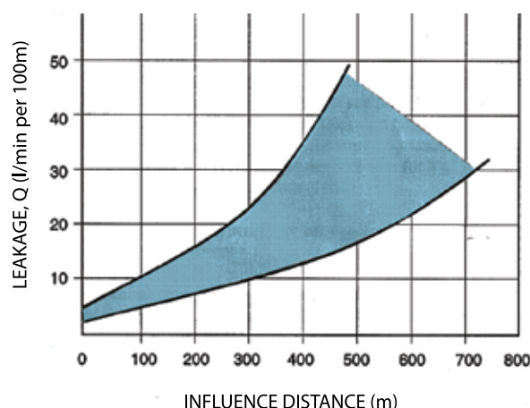
Figure 62. Influence distance in relation to inflow level
